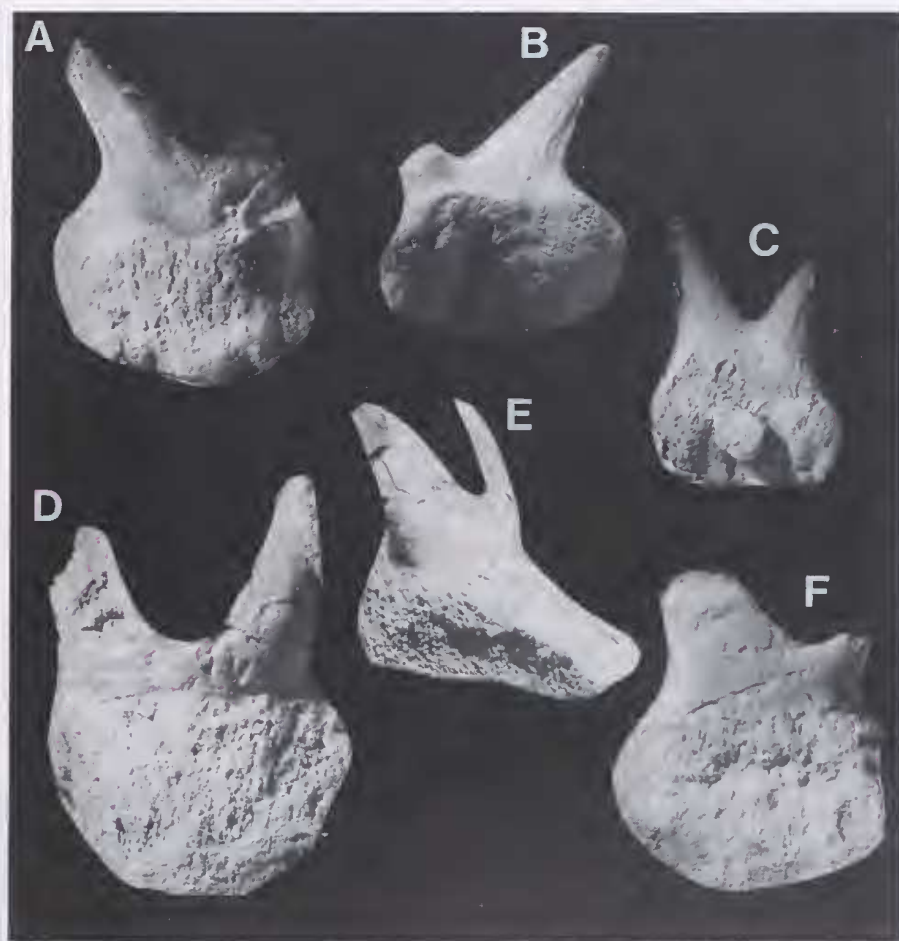
Figure 5 Portalodus bradshawae gen. et sp. nov. A, WAM 94.2.8., labial view, X 4 . B, WAM 94.2.10., lingual view, X 4 (both from Portal Mountain, type locality). C, WAM 94.2.12., lingual aspect, slightly flattened to show basal view also, X 2, from "Gorgon's Head", Cook Mountains. D, E, Holotype WAM 92.3.60. X 4, D, labial view, E, left lateral view (Portal Mountain, type locality). F, WAM 92.3.65, labial view, from Fault Bluff, "fish hotel" B horizon. A-C are latex casts whitened with ammonium chloride, D-F are actual specimens (whitened).
